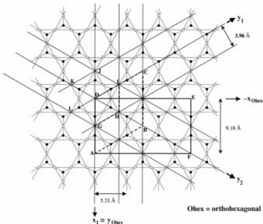
Figure 4. Schematic representation of the relationships between the silicate surface and planes of organic units. The hexagonal cell ABCD and the orthohexagonal cell ADEF of HDTMA-vermiculite are shown in relation to the smaller hexagonal cell DGHI.
